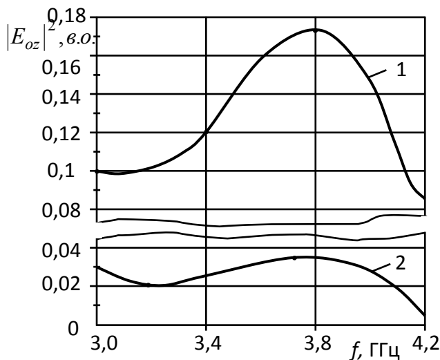
Fig. 1. The square of amplitude of EMF electric component |E_{0z}|^2 versus frequency response f for a pig leg: 1 – in bone marrow area; 2 – in bone tissue area
