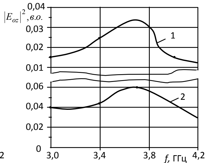
Fig. 2. The square of amplitude of EMF electric component |E_{0z}|^2 versus frequency response f for a cow leg: 1 – in bone marrow area; 2 – in bone tissue area
